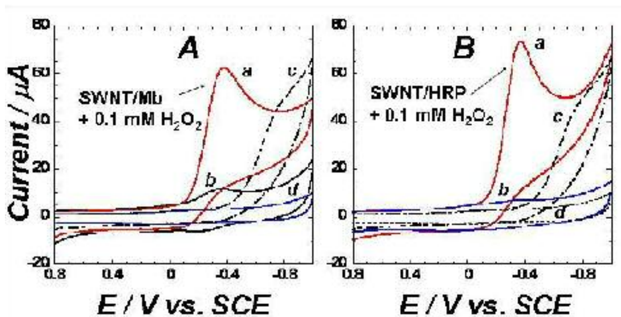
Figure 2-3. Cyclic voltammograms at 0.3 \text{ Vs}^{-1} for (A) SWNT/Mb and (B) SWNT/HRP after injecting 0.1 \text{ mM H}_2\text{O}_2 (a), SWNT/protein in anaerobic buffer pH 7.0 (b), SWNT control + 0.1 \text{ mM H}_2\text{O}_2 (c) and SWNT control in anaerobic buffer pH 7.0 (d).
