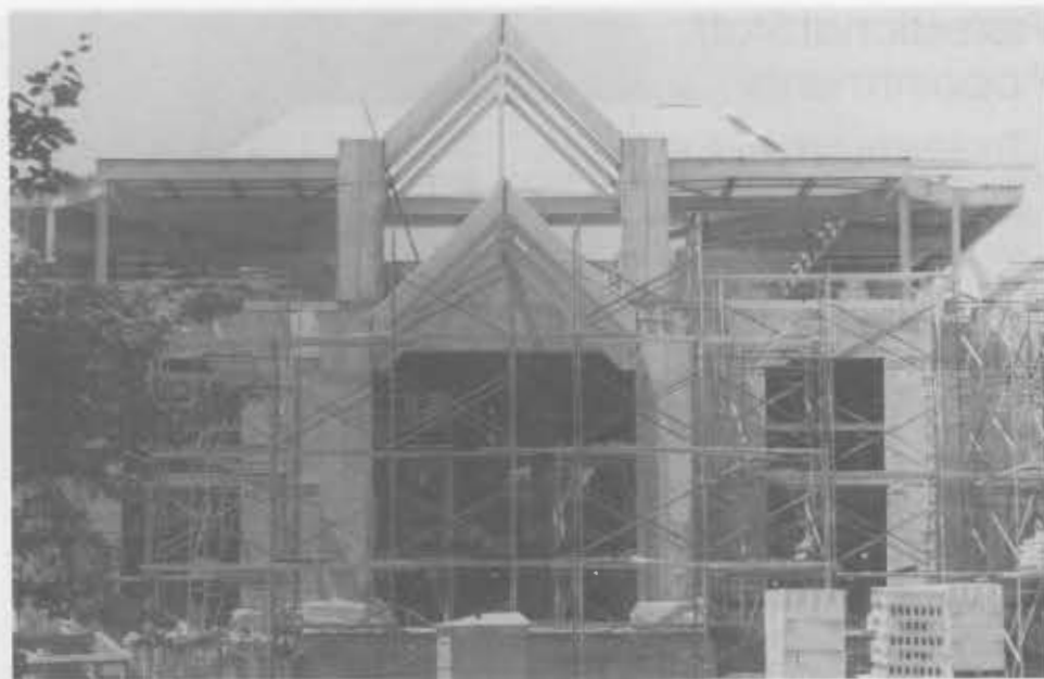
Construction of the new library progresses. The sandy gray rock-face granite exterior and lead-coated copper roof will echo turn-of-the-century design prevalent in buildings around campus. The entrance of polished granite in two shades of gray will pave the way to gray and dark blue carpeted floors and stairways. Traditional upholstered furniture, dark stained oak tables, barrister chairs, shelving and trim will harmonize with the historic character throughout the College.
